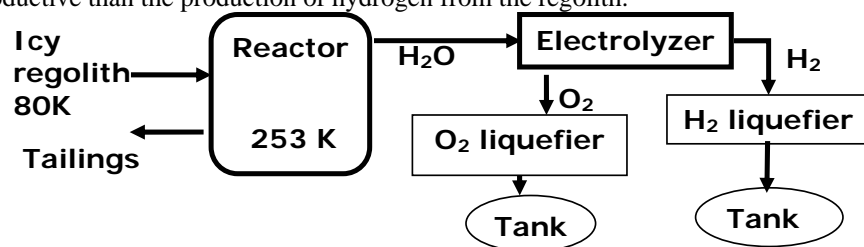
Figure 12. Schematic of a process to extract hydrogen from typical lunar regolith. Note the very large quantities of regolith that must be processed to extract the small amounts of H 2 and O 2 . The system would have to be more complex, to deal with the other volatiles present in the lunar regolith, but these would also become useful byproducts.
