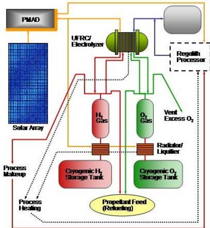
Figure 13. Schematic Regenerable Fuel Cell. During the day, energy from the solar array allows water (upper right) to be introduced into the electrolyzer, producing hydrogen and oxygen. At night, the process is reversed, producing energy and reconstituting the water.
