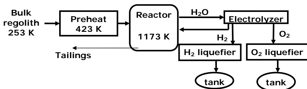
Figure 11. Schematic of a process to extract hydrogen from typical lunar regolith. Note the very large quantities of regolith that must be processed to extract the small amounts of H 2 and O 2 . The system would have to be more complex, to deal with the other volatiles present in the lunar regolith, but these would also become useful byproducts.
