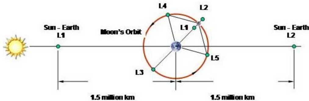
Figure 3. Schematic view of Earth–Moon Lagrangian points of gravitational stability in the Sun–Earth and Earth–Moon system.
