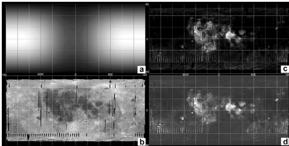
Figure 9. Simple cylindrical projections (left side of images corresponds to 180 W longitude; 30-degree grid shown, resolution is 0.25°/pixel) of (a) solar wind fluence model, (b) Clementine 750-nm mosaic; (c) \text{TiO}_2 abundance map from Lucey et al. (1996) Not in reference list. displayed from 0 to 6 wt. Percent; and (d) ^3\text{He} abundance map displayed from 0 to 10 ppb (from Johnson et al., 1999).
