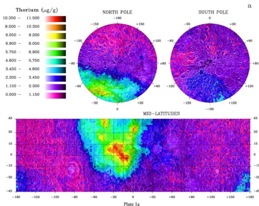
Figure 10. Lunar Prospector thorium concentrations. Thorium is most highly concentrated in the region surrounding Mare Imbrium on the lunar near side.
