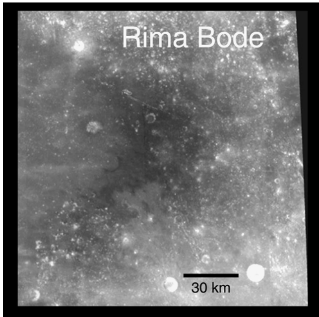
Figure 7. Clementine 750-nm images of dark pyroclastic deposits at Rima Bode.
