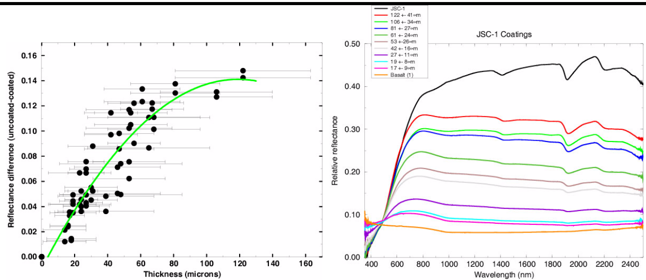
Figure 2. Reflectance differences between coated and uncoated samples as a function of coating thickness, showing a linear correlation until ~80μm thickness. Curve is quadratic fit to the data.
