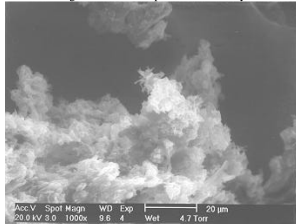
Fig 1A. Metallogenium mineral from Horse Tooth Reservoir in Fort Collins, Colorado. ESEM Photograph taken by Suzanne Douglas at the Jet Propulsion Laboratory.
