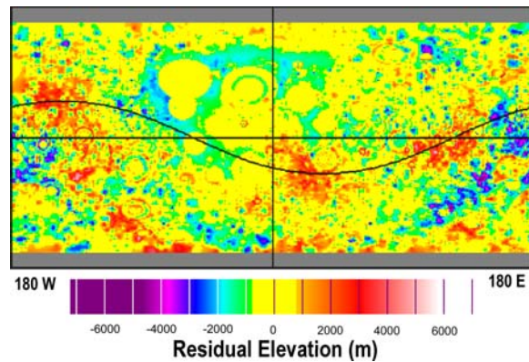
Figure 2: This geographic projection of the Moon shows the difference between the measured elevations and that of the models. The area within 12 degrees of the poles, where the LIDAR elevations are not accurate, are in gray. Two major anomalies are the Oceanus Procellarum depression (blue, northwest) and the three crustal deposits (orange, on a great circle with a pole at 65 N, 35 E).
