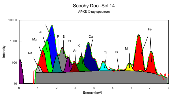
Fig.1 The X-ray spectrum of A-10 site – Scooby Doo. The appearance looks like a rock, but the analysis is more soil-like.
