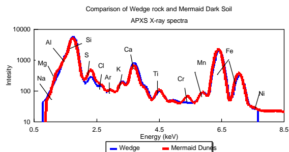
Fig.2 Comparison of X-ray spectra from a typical soil and a rock. Higher Mg, S and Cr on the soil is clearly visible as compared to the rock.
