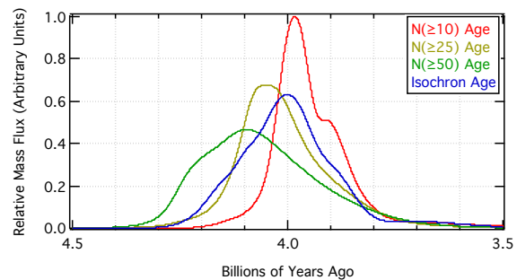
Figure 3: Curves are calculated the same way as ages from Fig. 2 except that each Gaussian for each crater has been scaled by D_{crater}^3 to approximate the mass of the impactor. The large basins have been excluded.
