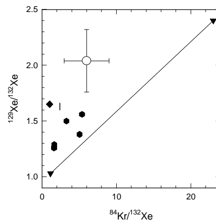
Figure 1: Plot of the ^{129}\text{Xe}/^{132}\text{Xe} isotopic ratio vs. the ^{84}\text{Kr}/^{132}\text{Xe} elemental ratio for various martian meteorites. Most shergottites (not shown) plot along the line connecting the martian atmosphere (upper right, measurement from EETA 79001) with Chassigny (lower left, potentially a sample of volatiles from the interior of Mars). Whole-rock nakhlite meteorites (solid symbols) have elevated ^{129}\text{Xe}/^{132}\text{Xe} ratios suggesting the presence of martian atmosphere, but their low Kr/Xe elemental ratios mean that if they did incorporate atmospheric gas, it was through a process that involved elemental fractionation. The iddingsite sample (open symbol) looks similar to the whole-rock nakhlites, and the absolute abundances in iddingsite are high enough to suggest that it is a major (if not the dominant) site of the atmospheric-like gases in nakhlites.
