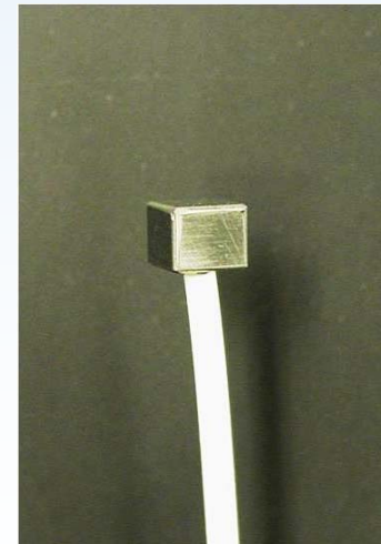
Fiber Optic Scintillation Detector (right)
