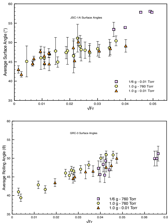
Figure 1: Measured surface angles for JSC-1A and GRC-3. Error bars indicate variance in the measurement sets. Uncertainty for some lunar (1/6-g) data is not available because each data point represents only one or two angle measurements.
