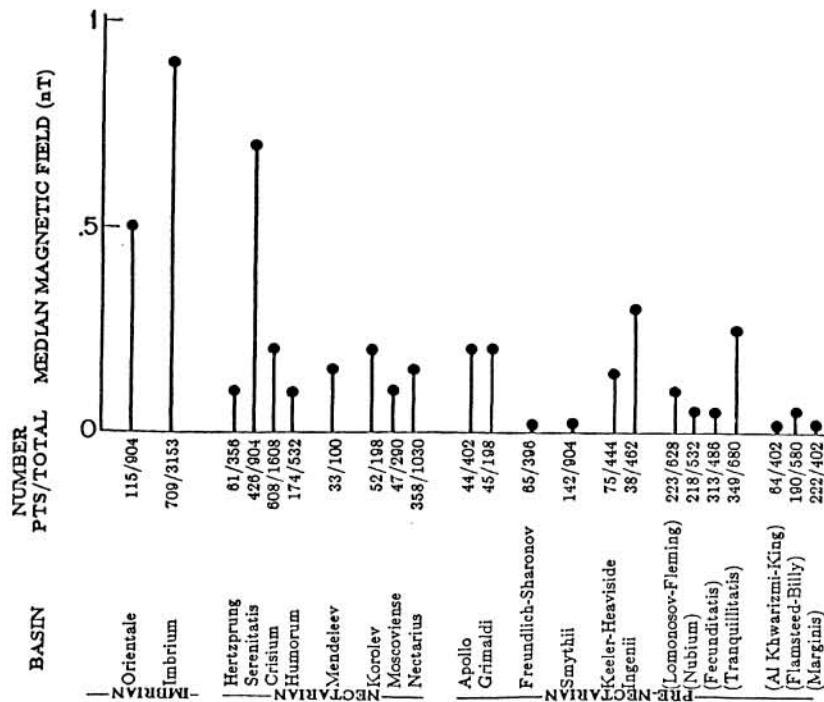
Figure 3. The median magnetic field for the antipodal regions of 23 impact basins. The number of samples and the total number possible for the antipodal region are given to provide an indication of the coverage.
