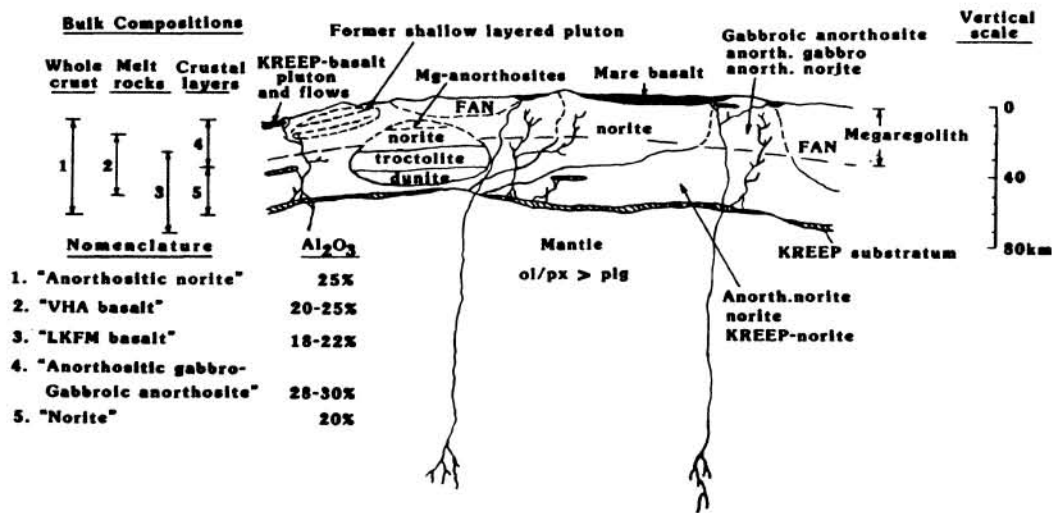
Fig. 1. Proposed model for the lunar crust. FAN refers to ferroan anorthosite. Provenance of bulk compositions indicated at left by arrows. See text for discussion.
