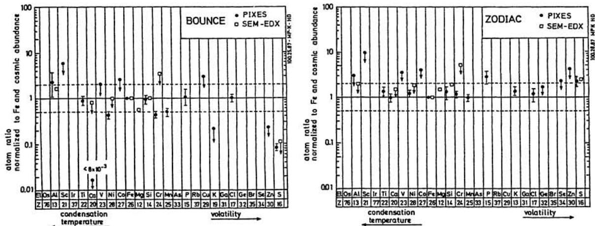
Fig. 1: Fe-normalized abundances of the elements in Bounce and Zodiac obtained by PIXES (this work) and SEM-EDX [8]. The elements are arranged according to decreasing condensation temperature [13]. Upper limits are given if the error exceeds 50 percent.
