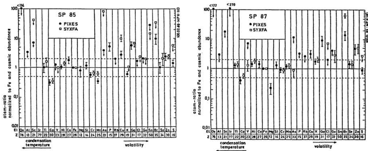
Fig. 2: Fe-normalized abundances of the elements in SP85 and SP87.
