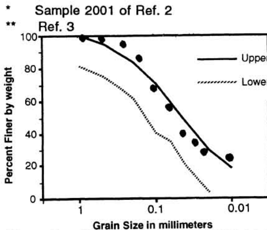
Figure 2. Size distribution of JSC-1 (dots) compared to lunar soil (Ref. 4).
