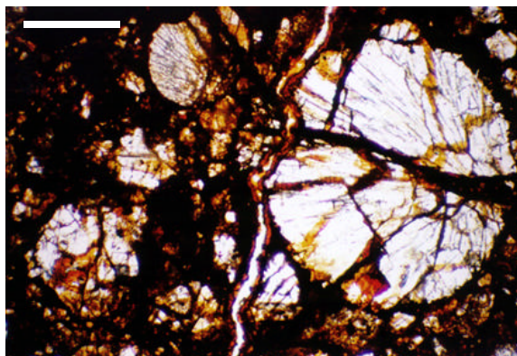
Fig. 2. Photomicrograph of Lea County 003 (Open nicol). Chondrules are partly weathered and replaced by brown alteration materials along cracks. Scale bar is 0.2 mm.
