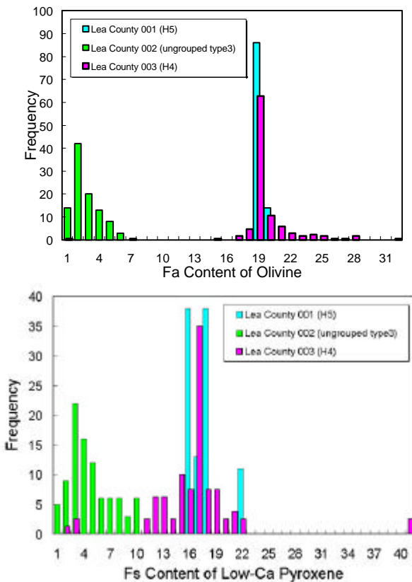
Fig. 3. Histograms of random analyses of olivine and low-Ca pyroxenes in Lea County 001, 002 and 003 chondrites. Lea County 003 is different from both Lea County 001 and 002. The total number of analyses for olivine and pyroxene in Lea County 003 are 169 and 80, respectively. Data for Lea County 001 and 002 are from Zolensky et al. [4].
