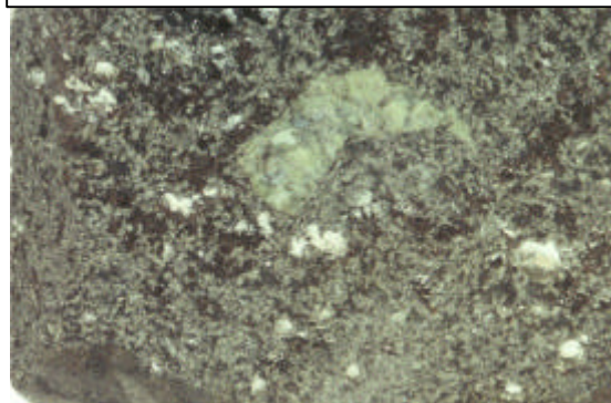
Fig.4: The largest olivinite encountered in D'Orbigny. Note the peculiar shape. (length is 3.7 cm).
