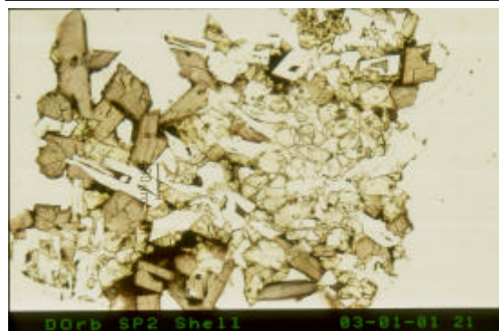
Fig.3: The bottom of a shell (granular) with druse augite crystals on top and bottom.
