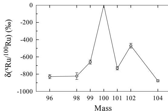
Figure 1: Ru isotopic composition in SiC grain L2 from Murchison indexed to the s -only isotope 100 Ru and normalized to a Ru terrestrial standard. Error bars are 2\sigma .
