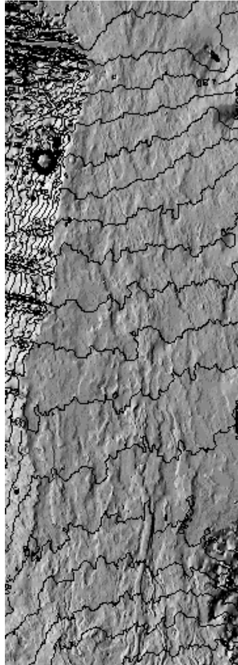
Figure 1. MOLA-derived elevation data for an area to the east of Pavonis Mons, with 100-m topographic contours. Note the overall coherence of lava flow directions to the local slopes.
