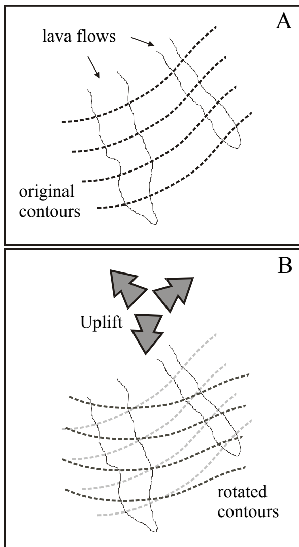
Figure 3. Deflection of topographic contours relative to lava flow directions in response to tectonic uplift. Similar changes in regional topography can also be caused by subsidence.
