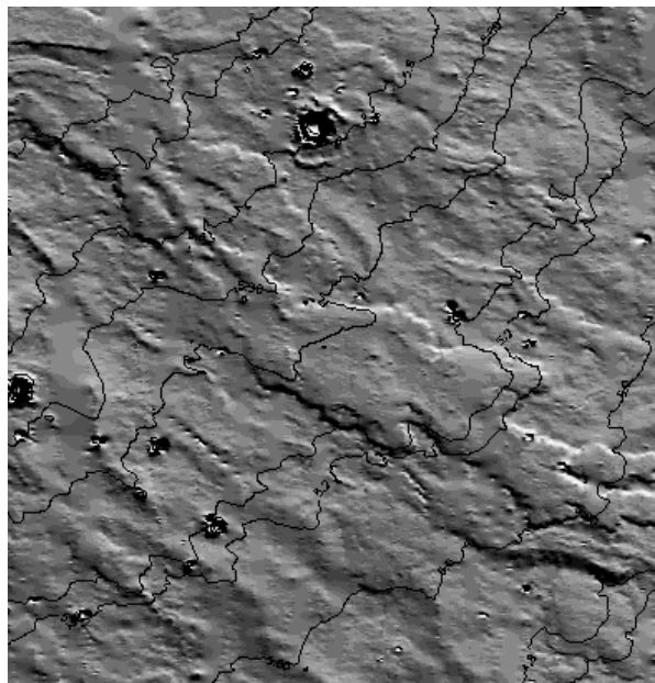
Figure 2. MOLA-derived digital elevation data and superimposed 200-m contours for an area to the north of Noctis Labyrinthus. Lava flow directions in this area are consistently deflected in a counter-clockwise direction relative to the regional topographic contours, and indicate post-emplacement deformation.
