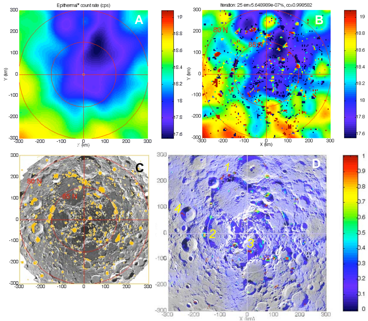
Fig. 1. (A) Smoothed epithermal neutron count rate map for the lunar north pole. (B) Deconvolved epithermal count rate map using constraints from a liberal shadow model. (C) Shadow model (orange) superimposed on a Clementine photomosaic. (D) WEH in wt% superimposed on the photomosaic. See text for numbers.
