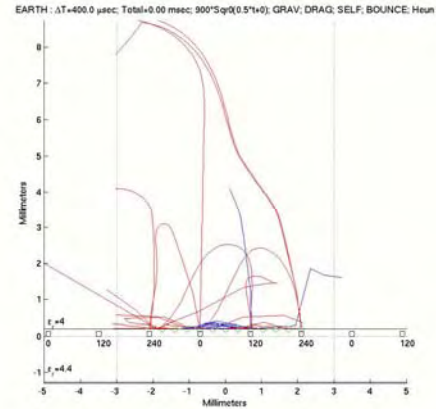
Figure 3. Trajectory calculation for 12 charged dust particles over 8 three-phase square signals, 900 volts.
