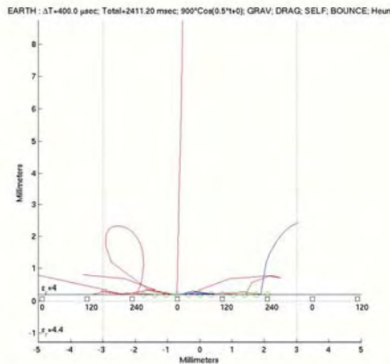
Figure 2. Trajectory calculation of 12 charged dust particles over 8 three-phase sine signals at 900 volts.
