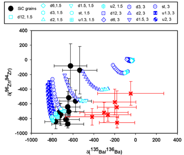
Figure 2. Two-element plot of Ba and Zr isotopic ratios in mainstream SiC grains compared with model predictions for 1.5 and 3 M_{\odot} carbon-rich AGB stars with solar initial metallicity (open symbols).
