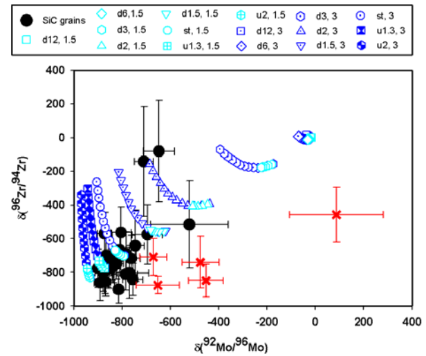
Figure 1. Two-element plot of Mo and Zr isotopic ratios in mainstream SiC grains compared with model predictions for 1.5 and 3 M_{\odot} carbon-rich AGB stars with solar initial metallicity (open symbols). Filled circles are individual grains within 2\sigma of predictions. Crosses are grains believed to have been contaminated with Mo but not Zr.
