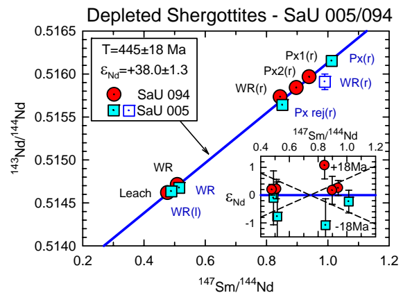
Figure 2. Sm-Nd data of SaU 005/094.
