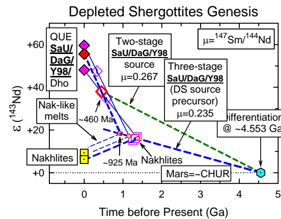
Figure 4. \epsilon_{Nd} vs. T(age) of dep. shergottites & nakhilites.
