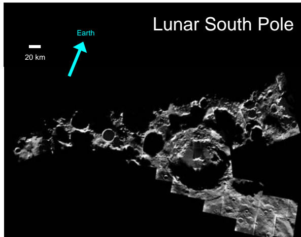
Fig. 1: SMART-1 /AMIE mosaic of the lunar South Pole . The pictures were taken between May 2005 and February 2006, during different phases of the mission.. at a distance of about 400 km, allowing medium-field (about 40 km across) and high-resolution views (40 m/pixel).
