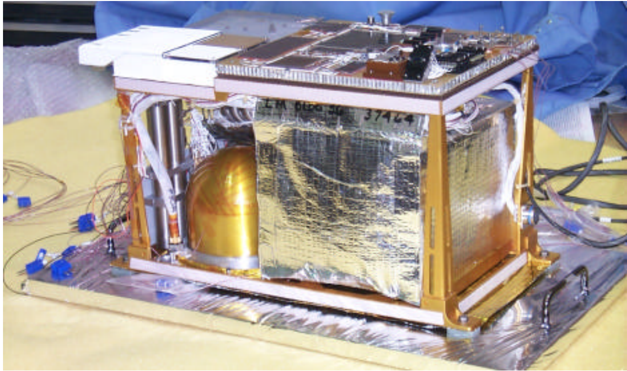
MIP Engineering Development Unit
