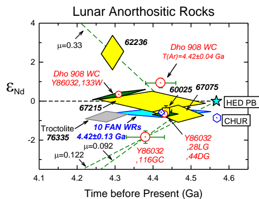
Fig. 2. (T, \epsilon_{Nd} ) diagram for lunar anorthosites, anorthositic clasts, and troctolite 76335.
