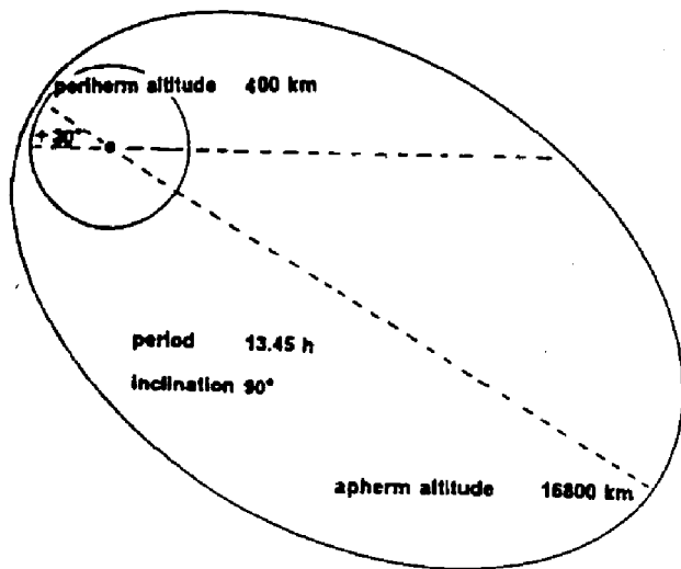
Fig.2. Mercury Orbiter operational orbit.
