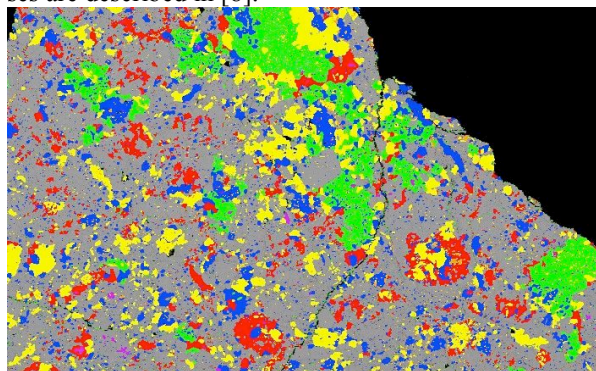
Figure 1. EMP element map portion of section of LAP 04840,30. Grey=olivine; green=orthopyroxene; red=plagioclase; yellow=amphibole; blue=opaques; orange=Ca-phosphate; purple=biotite.
