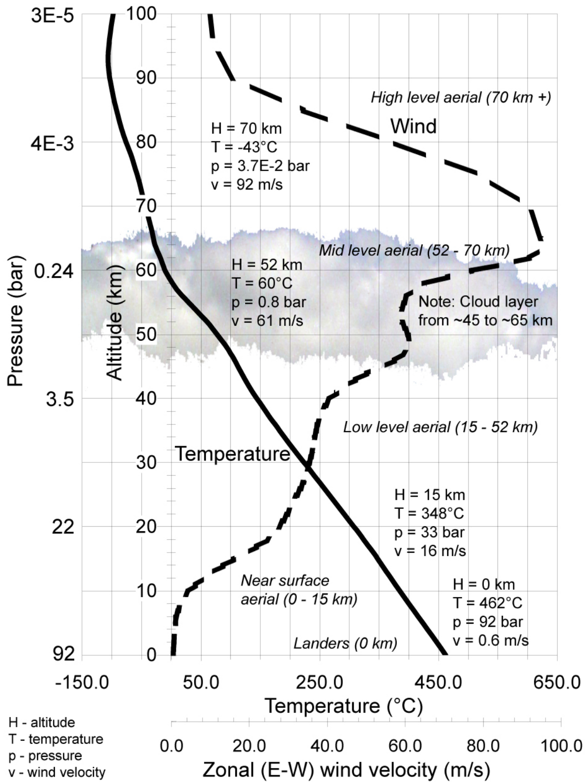
Figure 1: Pressure, temperature and wind conditions at Venus
