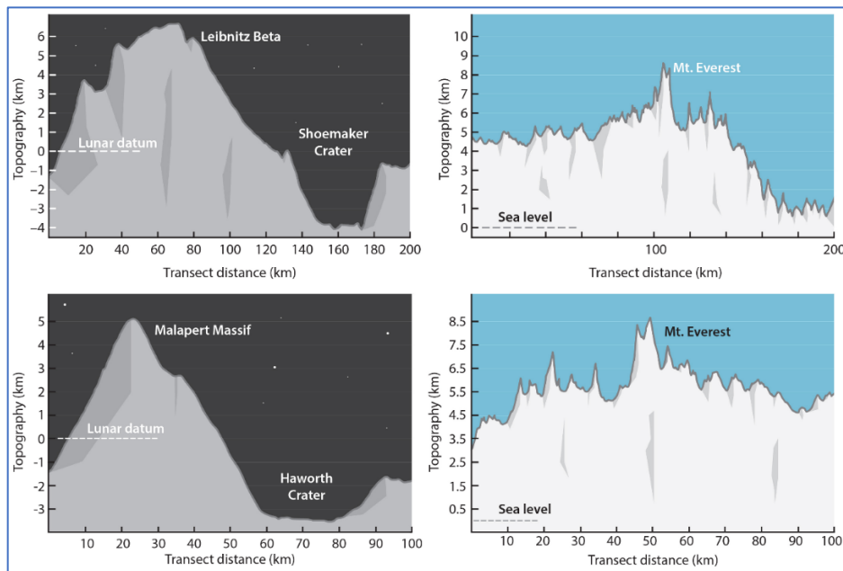
Figure 3. Topographic transects across the Moon's Leibnitz Beta massif and Shoemaker crater (top) and Malapert massif and Haworth crater (bottom) are compared with transects over Mt. Everest on Earth. The horizontal scales are 200 km (top) and 100 km (bottom). The change in elevation in the Leibnitz Beta transect exceeds 10 km and the elevation of Earth's Mt. Everest above sea level. The change in elevation in the Malapert transect exceeds 8 km, a value very close to the elevation of Earth's Mt. Everest. Illustration credit: LPI/CLSE.
