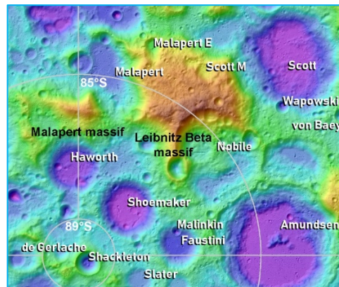
Figure 1. Topography from the south pole to the Malapert and Leibnitz Beta massifs. Both massifs occur within 6° of the south pole, which is the study domain for the Artemis III landing. Detail from [8].
