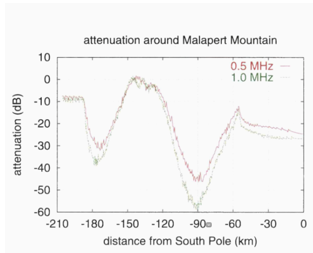
Figure 1: Simulations show that terrestrial radio waves, even at very low frequencies, would be attenuated by 5 orders of magnitude in the region directly beyond Malapert Mountain. Taken from [5].
