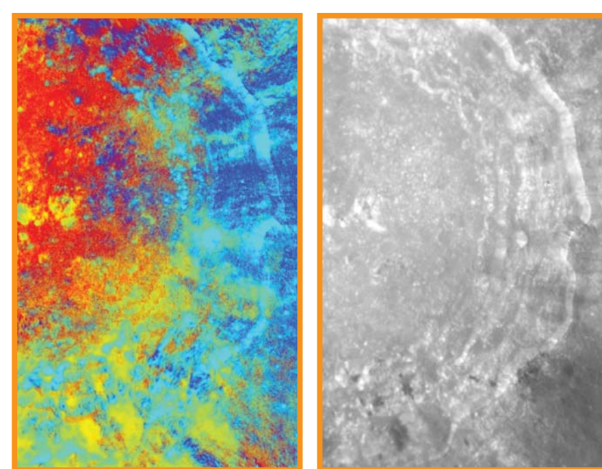
Copernicus Crater as imaged by spectrometers onboard the Clementine spacecraft. The left side combines data collected through three different color filters. The resulting image represents different rock types and shows the geologic complexity of the crater. For example, the green-yellow areas have rocks with higher iron content. The right side shows the features in a single wavelength of 750 nanometers. Image processing by Brown University.
