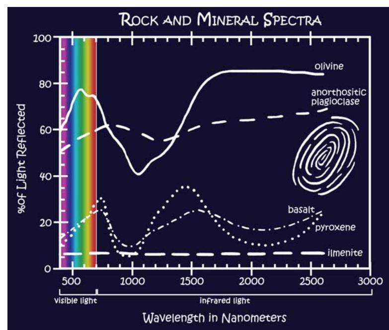
This graph shows reflectance spectra of several minerals common on Earth and the Moon, and a lunar basalt. The spectral fingerprint of the basalt is a result of combining different amounts of the mineral spectra. Its shape is similar to the shape of the pyroxene spectrum. Indicating that the basalt contains a large amount of pyroxene. The basalt also contains plagioclase, and minor amounts of olivine and ilmenite. Ilmenite, a dark mineral, has a low reflectance; when light strikes this mineral most is absorbed and little is reflected. The presence of ilmenite in basalt contributes to the low reflectance of basalt.
