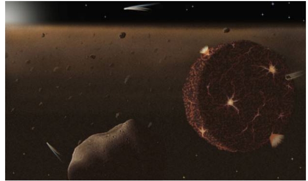
Planets Form
