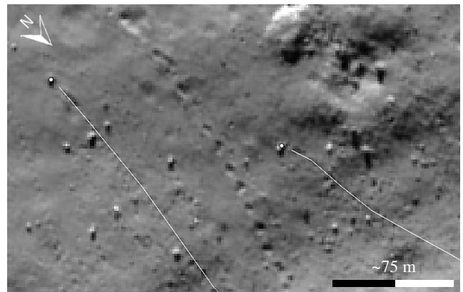
Fig 2. Rockfalls in Shackleton crater, slope dips to the upper left.
