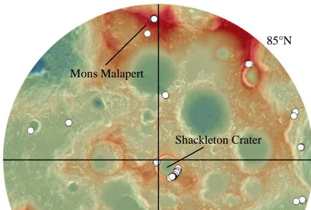
Fig. 1. Boulders with tracks at the South Pole; on LOLA DEM.
