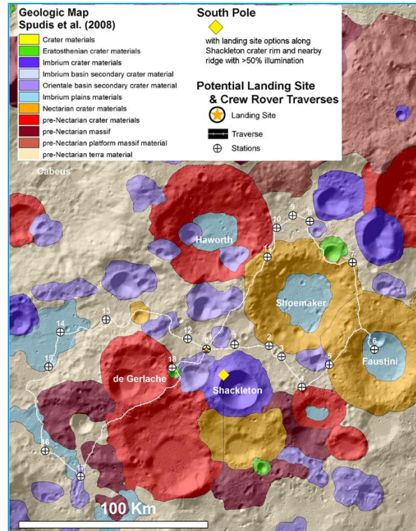
Figure 1. Geologic map with South Pole landing site, suitable for both crew and rover-facilitated traverses, plus a second landing site with rover-facilitated traverses of PSRs. Modified after Spudis et al. (2008) and Allender et al. (2019).
