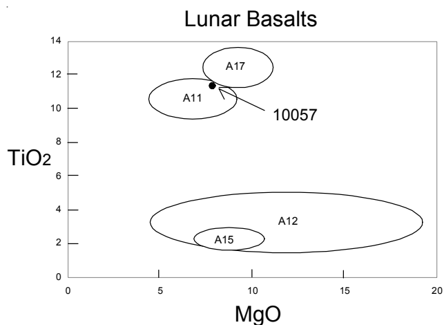
Figure 4: Composition of lunar basalts showing position for 10057 (data from table 1).
