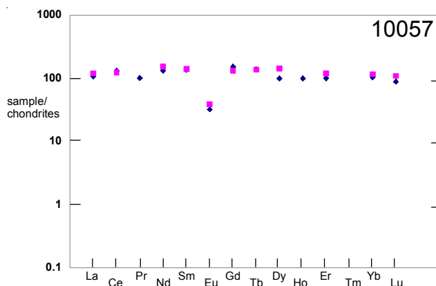
Figure 5: Normalized rare-earth-element diagram for high-K basalt 10057 (data from Wanke et al. 1970 and Haskin et al. 1970 only).
