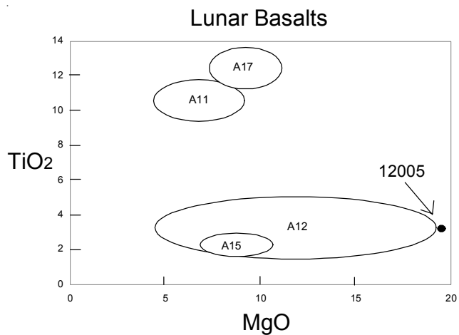
Figure 7: Composition of lunar basalts showing relative position of 12005.
