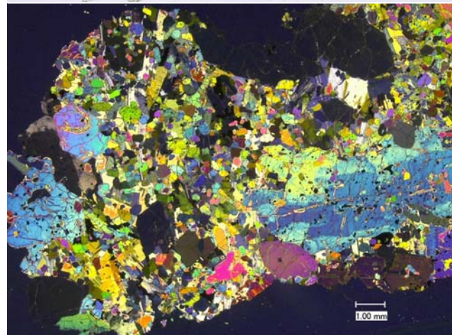
Figure 2b: Photomicrographs if thin section 12005,57 by C Meyer @ 20x. See also video file.
