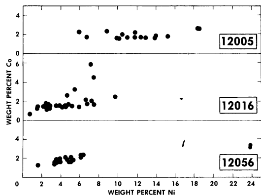
Figure 6: Composition of metal grains in lunar samples (from Dungan and Brown 1977).
