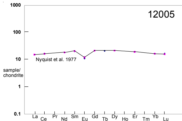
Figure 8: Normalized rare-earth-element composition diagram (data from Rhodes et al. 1977 and Nyquist et al. 1977).
