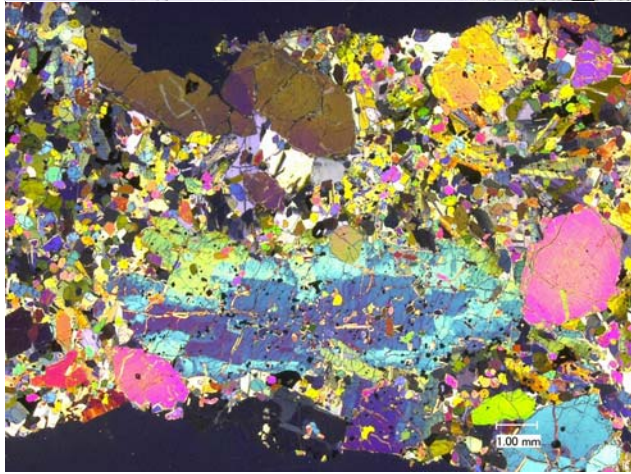
Figure 2a: Photomicrographs of thin section 12005,57 showing large zoned pyroxene.
