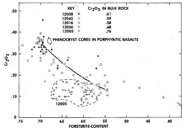
Figure 4: Trace element content of olivine in Apollo 12 samples (by Dungan and Brown 1976).
