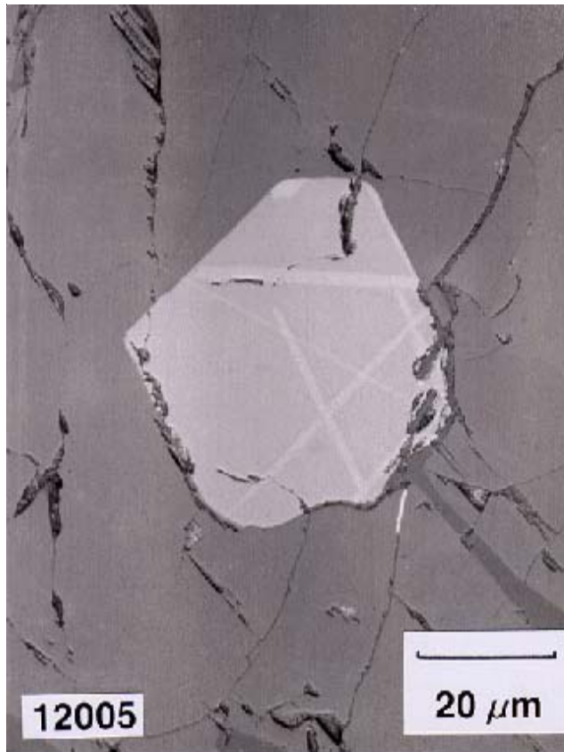
Figure 5: Olivospinel with exsolved ilmenite in 12005.
