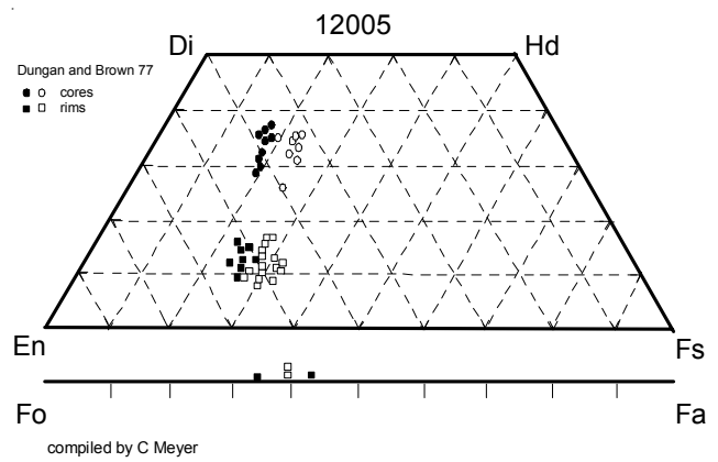
Figure 3: Pyroxene and olivine composition for 12005 (from Dungan and Brown 1977). Mafic minerals are relatively unzoned and there are two distinct pyroxenes.
