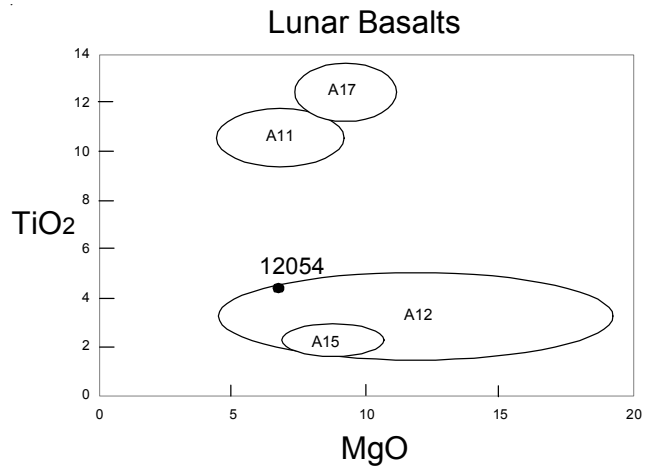
Figure 4: Composition of 12054 compared with that of other lunar basalts.
