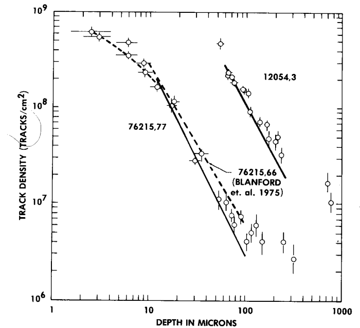
Figure 7: Solar flare track density as function of depth in glass on 12054 (from Morrison and Zinner 1977).
