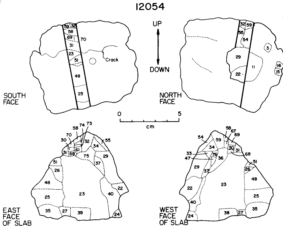
Figure 11: Cutting diagram for 12054 showing position and orientation of slab (from Hartung et al. 1978).
