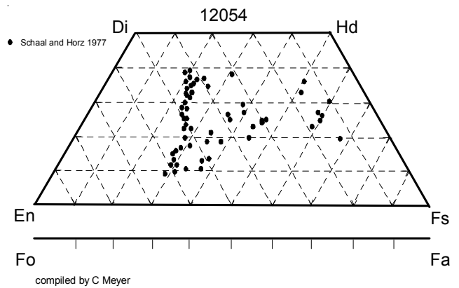
Figure 3: Pyroxene composition diagram for 12054 (from Schaal and Horz 1977).
