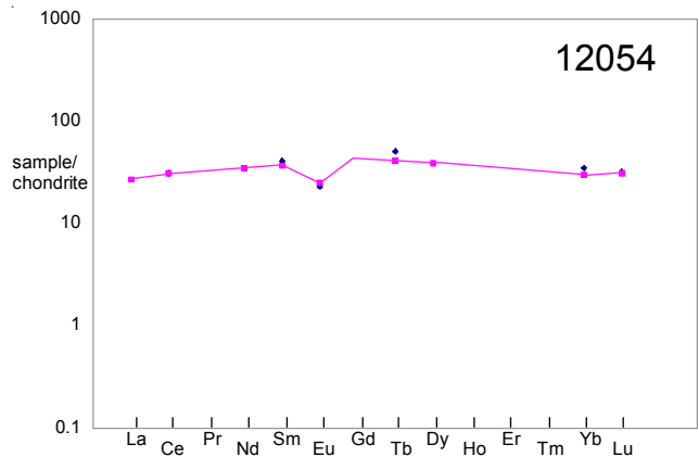
Figure 5: Normalized rare-earth-element diagram for 12054 (data from Neal et al. 1994 and Rhodes et al. 1977).
