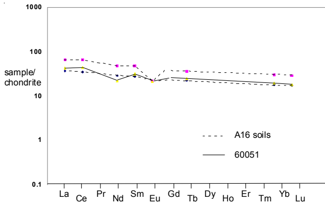
Figure 3: Normalized rare-earth-element diagram for Apollo 16 soils with 60051.
