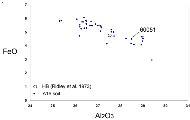
Figure 4: Chemical composition of Apollo 16 soil with average composition of 'highland basalt' (glass) and 60051.
