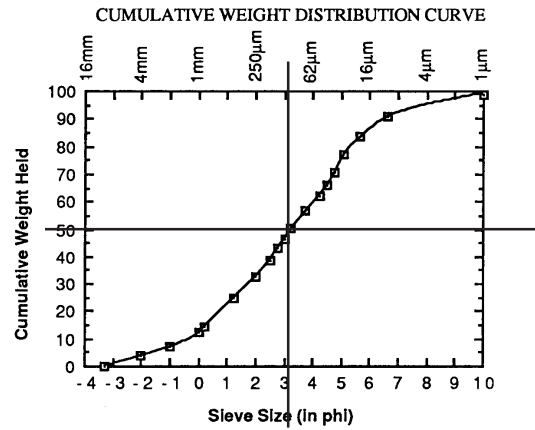
Figure 5: Comparison with friable ferroan anorthosites found in same bag.
