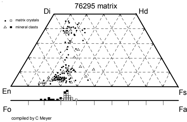
Figure 4: Composition of pyroxene and olivine in matrix of 76295 (data replotted from Phinney 1981).
