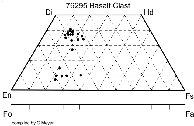
Figure 5: Composition of pyroxene and olivine in basalt clast within 76295 (data replotted from Phinney 1981).
