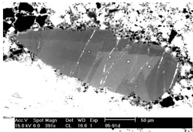
Figure 9: Back scattered electron image of large zircon grain in 76295 - called "arrowhead" by Pidgeon et al. 2006.
