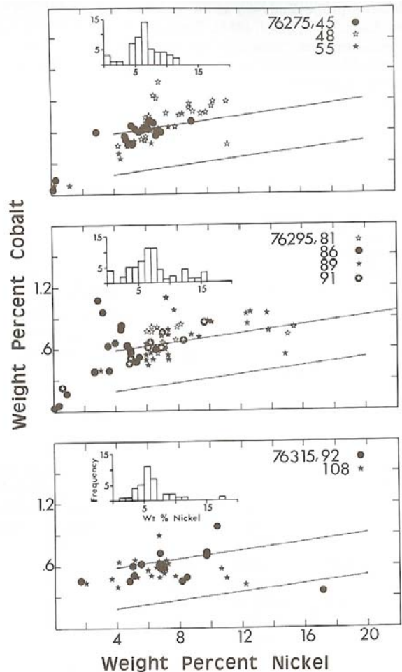
Figure 7: Ni and Co content of metal grains in 76295 (Misra et al. 1976).
