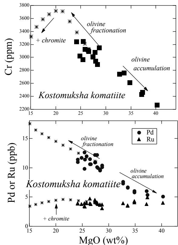
Figure 1: Cr, Ru and Pd trends with MgO in the Kostomuksha komatiite suite (from [12]). Major element modelling of crystal fractionation of the proposed Kostomuksha parent liquid [12] using the MELTS program [20] is coupled with new partitioning data. Asterisks indicate the calculated trends using the major element results, and D(\text{Ru}) and D(\text{Pd}) olivine/melt and chromite/melt measured here.
