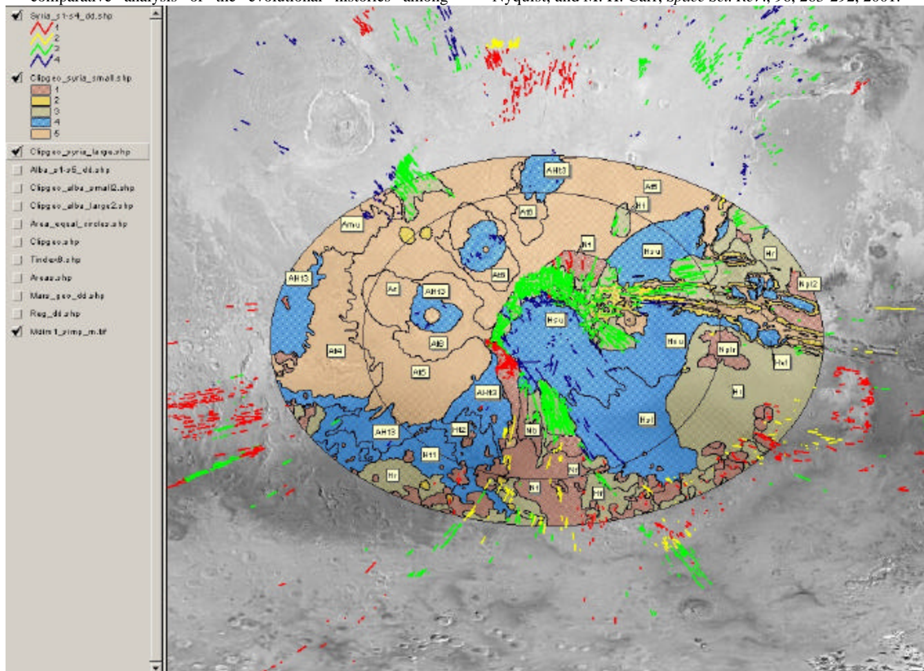
Figure 1) GIS-based Syria Planum faults projected onto geological units of Scott and Tanaka (1986) [3]. Colored faults and geologic map unit polygons correspond (color coded) to major stages of Tharsis geologic activity of Anderson et al. (2001) [1] and Dohm et al. (2001) [4,5].
