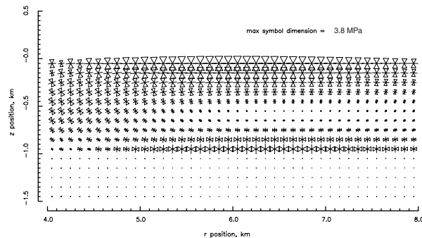
Figure 2: Close-up of the same simulation as shown in Fig. 1, at the same time, illustrating the principal stresses in the brittle upper layer. Pairs of triangles represent compression and lines represent extension. The size of the symbol scales with the magnitude of the stress, the largest symbol here is 3.8 MPa.
