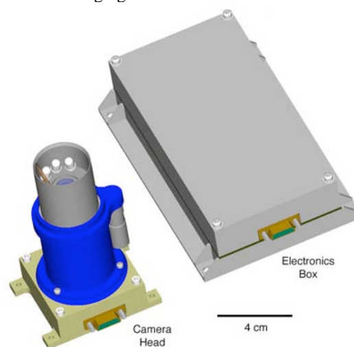
Fig. 1. Rendering of MSL MAHLI camera head and separate electronics box.
