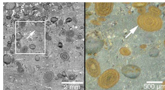
Fig. 3. Example of color and resolution working together, in this case to permit discrimination of different colors (translating to different composition) and concentric zoning (arrow) in goethite/chamosite ooids in a cut (analogous to the MSL abrasion tool) sample of late Devonian Saverton Shale from Iowa. At left is a 30 \mu\text{m}/\text{pixel} grayscale view (similar to MER MI); at right, a 12.5 \mu\text{m}/\text{pixel} color view of the area outlined by the white box on the left.
