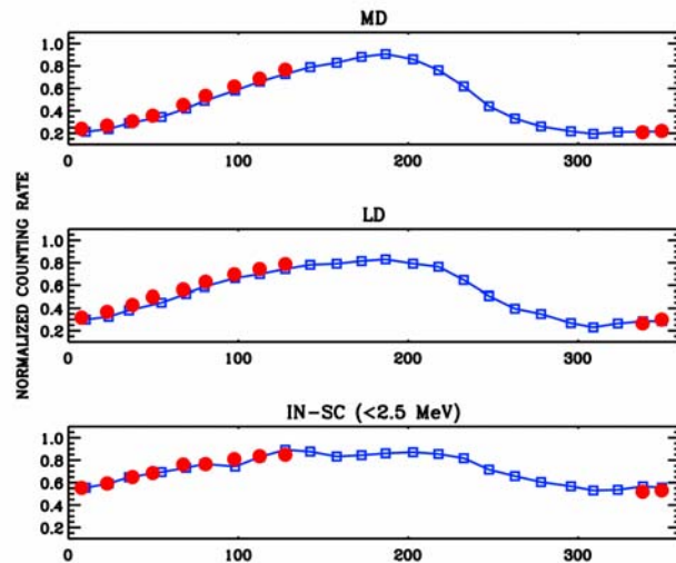
Fig. 2. Seasonal curves of neutron flux in different energy bands for southern polar region 80S-90S. The Y axis corresponds to the normalized counting rate in different HEND detectors and X axis describes the martian seasons measured by L_s . The top and middle graphs are created for MD and LD HEND detectors (epithermal neutrons) and the bottom graph corresponds to observations in soft channels of IN-SC detector (fast neutrons). The blue color was used for illustration of data points of the previous martian year and red color corresponds to observations performed during current martian year.
