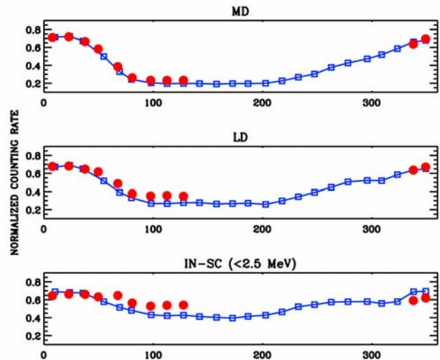
Fig. 1. Seasonal curves of neutron flux in different energy bands. The Y axis corresponds to the normalized counting rate in different HEND detectors and X axis describes the martian seasons measured by L_s . The top and middle graphs are created for MD and LD HEND detectors (epithermal neutrons) and the bottom graph corresponds to observations in soft channels of IN-SC detector (fast neutrons). The blue color was used for illustration of data points of the previous martian year and red color corresponds to observations performed during current martian year.
