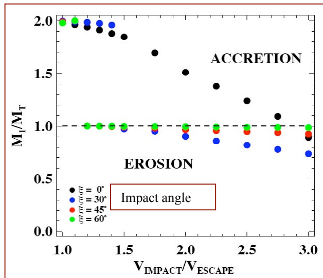
Mass of largest remnant normalized to initial largest mass, versus impact velocity normalized to escape velocity, for impactors half the mass of Mars-sized 30 wt% Fe targets.
