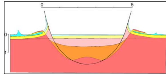
Fig. 1. Excavation phase and onset of central uplift (not confirmed). Target stratigraphy is indicated by paler shades (water: blue, sediments: yellow, crystalline: pink). Note dip of basement and deepening of seawater towards the south (left).
