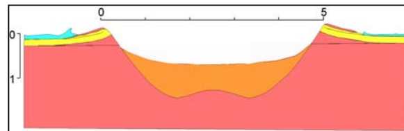
Fig. 2. Return of seawater. Due to the situation given in Fig. 1, the southern rim will immediately collapse. This brings on the situation in Fig. 3.
