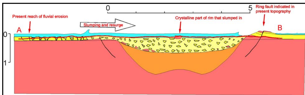
Fig. 3. Rim collapse occurs due to resurge of seawater and weakness of the southern rim. The collapse causes large-scale block slumping of poorly consolidated, fluidized sediments outside the crater. This is only occurring in the southern sector resulting in a horseshoe-shaped rim. A is south, B north.
