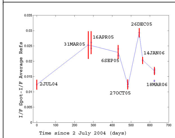
Fig. 2 Reflectance change at 2.02 \mu\text{m} Jul 04-Mar 06
