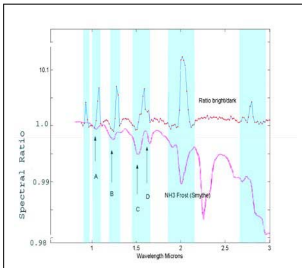
Fig 4 a. The \text{NH}_3 frost features are seen in the ratio at A=1.05 \mu\text{m} , B=1.24 \mu\text{m} , C=1.52 \mu\text{m} , and D=1.65 \mu\text{m} .
