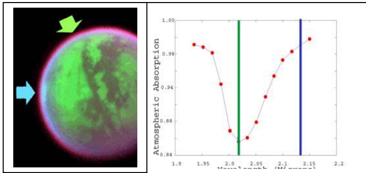
Fig 3. Left-RGB image of Fig 1. G (2.02 \mu\text{m} ) is at the center of the methane window. B (2.13 \mu\text{m} ) is at the band wing and shows the elevated cloud. R is 2.4 \mu\text{m} where \text{CH}_4 is completely opaque. Right- Titan's spectrum, 1.94-2.16 \mu\text{m}
