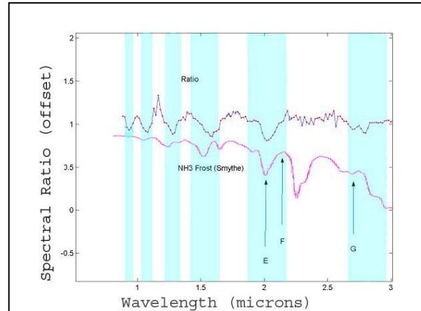
Fig4b. The ratio is divided by the normalized spectrum of the background to effect different amount of methane haze correction. This displays the \text{NH}_3 absorption features E=2.01 \mu\text{m} , F=2.13 \mu\text{m} , and G=2.69 \mu\text{m} .
