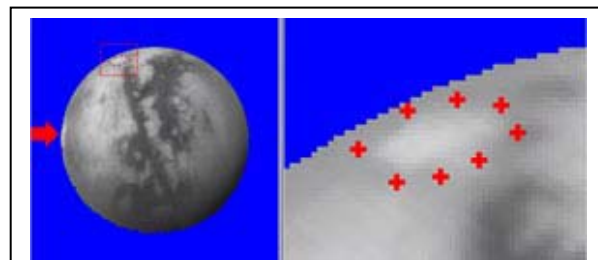
Fig. 1. Left -VIMS composite image at 2.02 \mu\text{m} for the 25Dec05 flyby (N is to the left) . Right-Enlargement of area enclosed by the red box on left. A cloud is indicated (red arrow).
