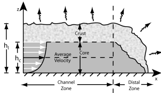
Fig 2. LEVEED FLOW CARTOON (FROM [3])
