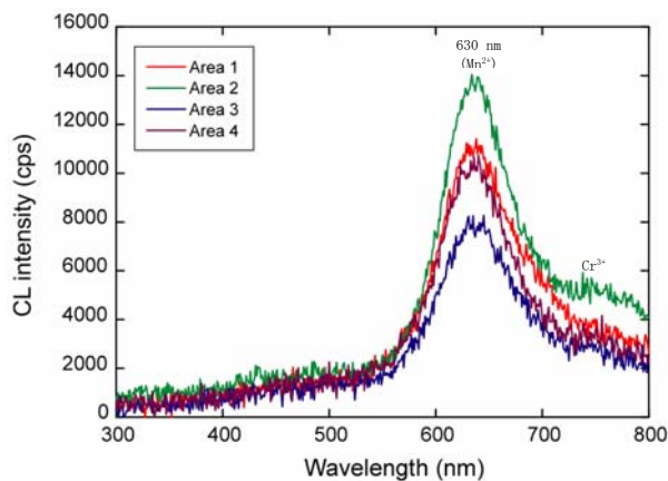
Figure 3. CL spectra of four areas containing a dominant broad band centered at around 630 nm.
