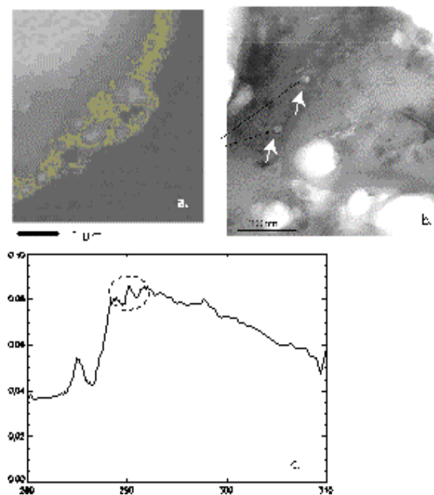
Figure 1: STXM image (a) of a fragment from Stardust Track 16 and the spectrum from the area of this image highlighted in green. The absorption peak near 290 eV (circled) is consistent with carbonate. TEM image of a fragment from Stardust Track 1 (b) also shows small carbonate (at arrows).
