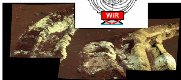
Fig. 1 WIR concept and the sulfate-rich soils excavated by the wheels of Spirit rover
